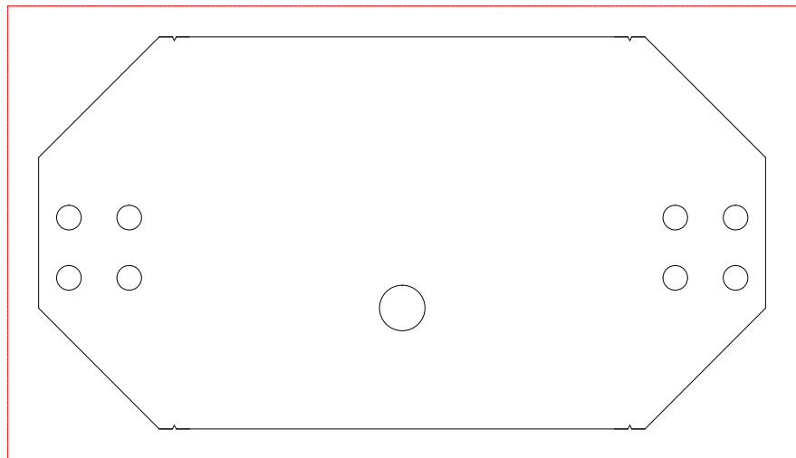
4 PARTS / PLATE 10 MM
